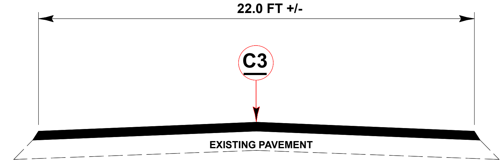
TYPICAL SECTION # 4 MAP(S) # 9
