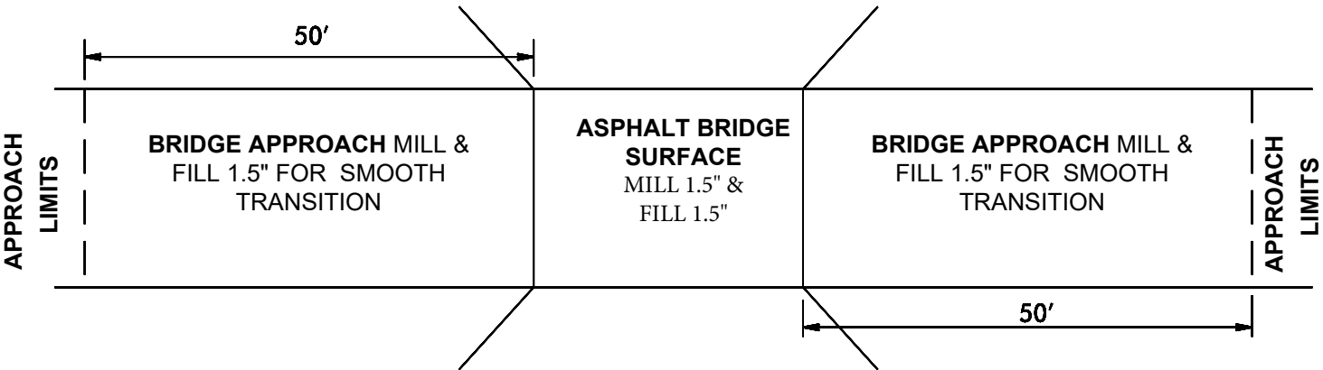
DETAIL FOR MAP # 3 / STRUCTURE # 0041
